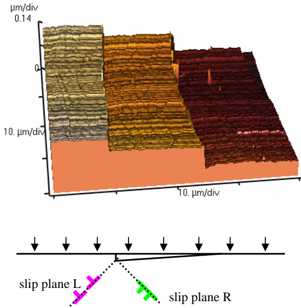
Figure 1 – An Atomic Force Microscope image of a cleaved LiF single crystal. The surface ledges, under contact, will emit dislocations along certain slip systems, as shown schematically.
