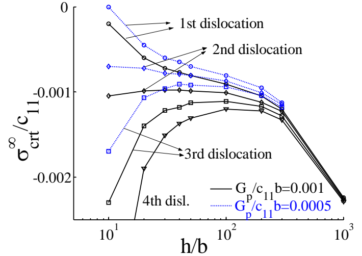
Figure 2 – Critical loads for dislocation nucleation are plotted against the step height h/b (normalized by b , the magnitude of Burgers vector). This plot only considers the slip plane L.
